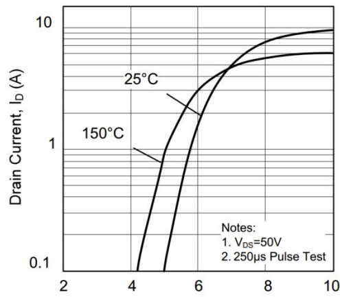
4. Transfer Characteristics
