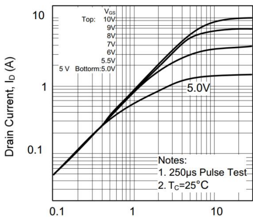
3. On-State Characteristics
