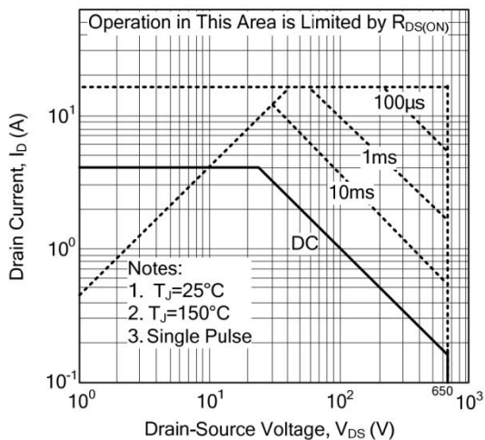
5. Safe Operating Area
