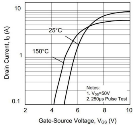
4. Transfer Characteristics
