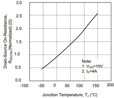
2. On-Resistance Junction Temperature
