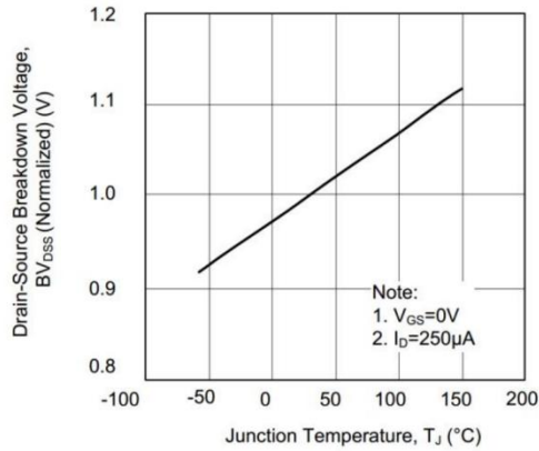
1. Breakdown Voltage Variation vs. Temperature
