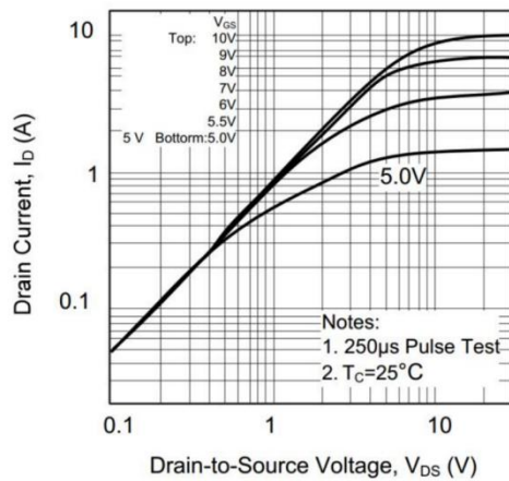
3. On-State Characteristics
