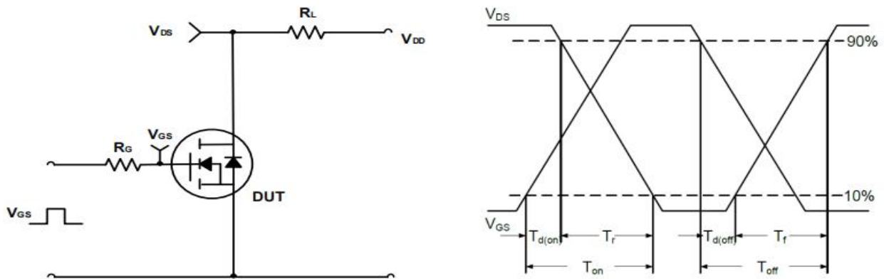
Figure B. Switching Test Circuit & Waveforms
