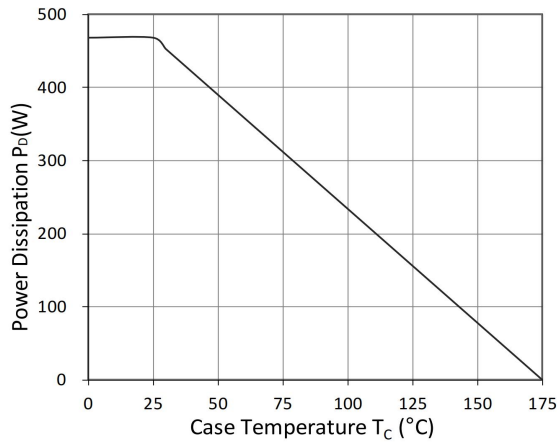
Figure 9. Power Dissipation
