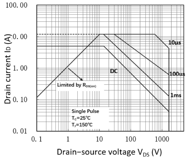
Fig.13 Safe Operating Area
