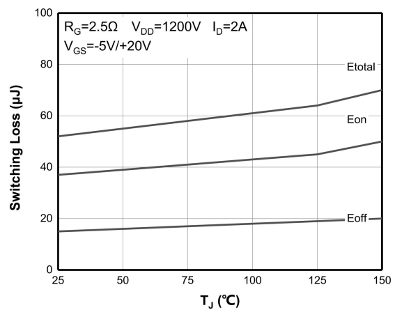
Fig.12 Clamped inductive switching energy vs. temperature
