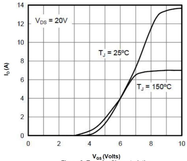
Figure 2: Transfer Characteristics
