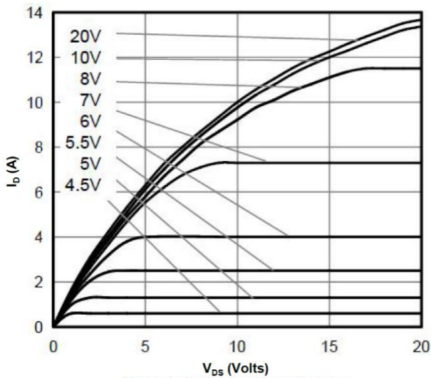
Figure 1: On-Region Characteristics
