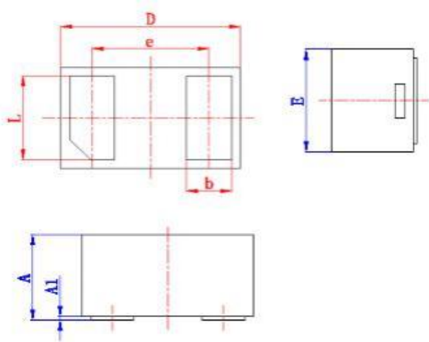
DFN1006-2L
